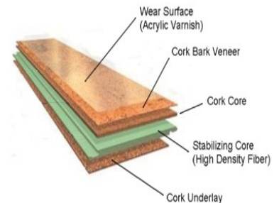
Sample Cork Floor Construction
